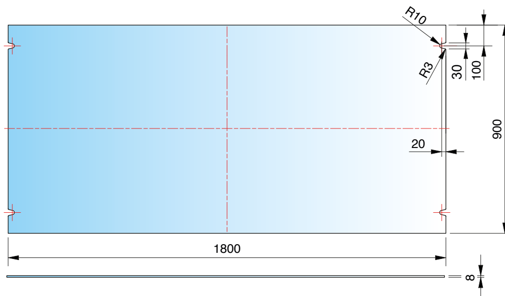
Standardabmessung standard dimension
